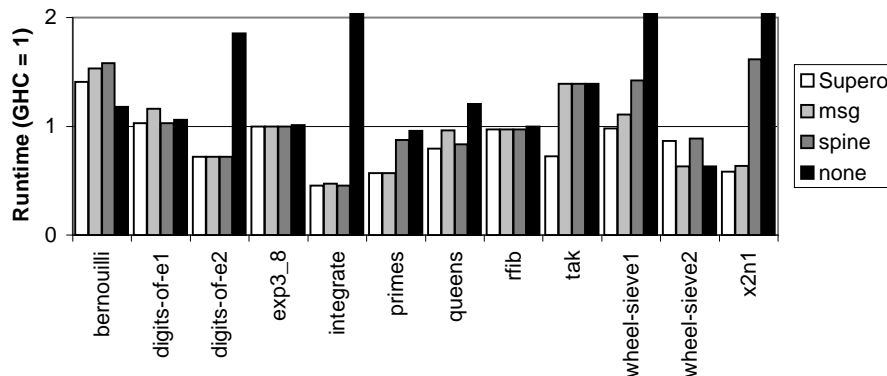
Supero uses the \bowtie generalisation method; msg uses the msg function for generalisation; spine applies no generalisation operation; none never performs any inlining.
